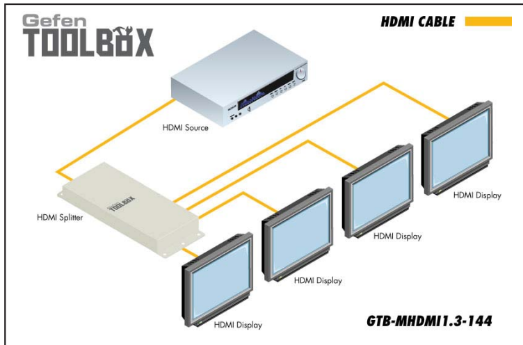
Wiring Diagram for the 1:4 Splitter for HDMI 1.3
